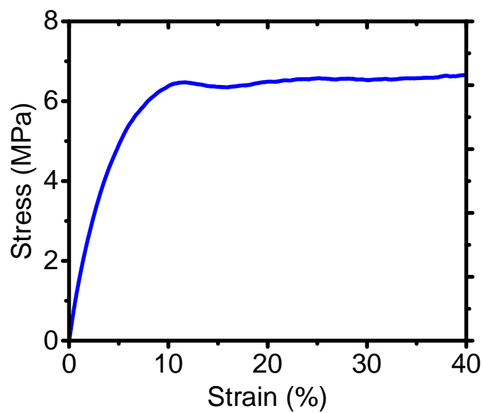
Figure S10 Stress-Strain curve for PEVA (VA content=5%).
