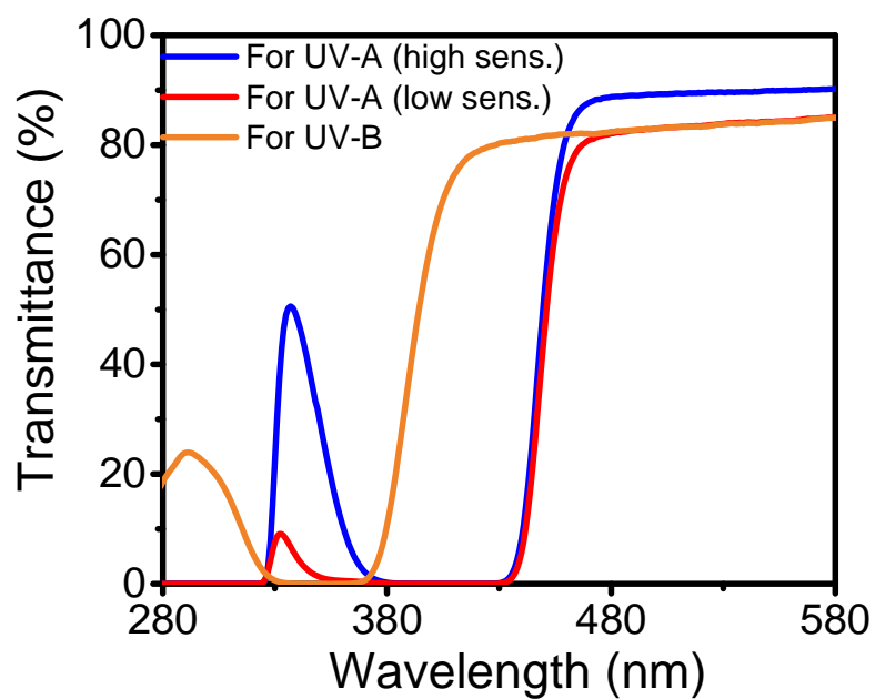
Figure S13 UV-vis transmittance for UV absorptive filters in butterfly designs for the integrated system demonstration.
