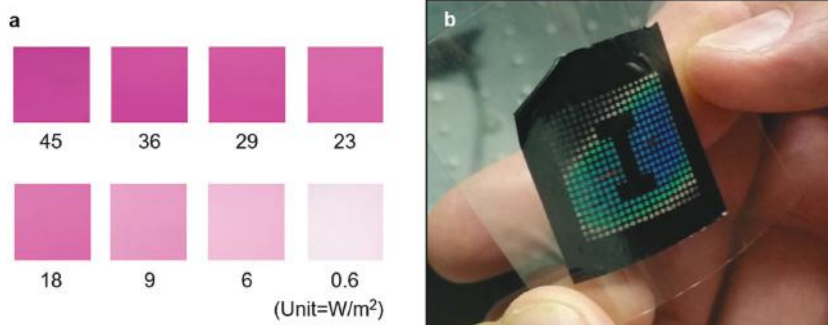
Figure 5. Images of the color response of stretchable materials for UV radiometry and the operation of a liquid crystal based colorimetric temperature sensor. a) Digital images of the UV colorimetric radiometer material captured just after UV-A exposure at intensities of 45, 36, 29, 23, 18, 9, 6, 0.6 \text{W m}^{-2} . b) Image of a patterned pixel array of thermochromic liquid crystal formed by screen printing on a film of PET.
