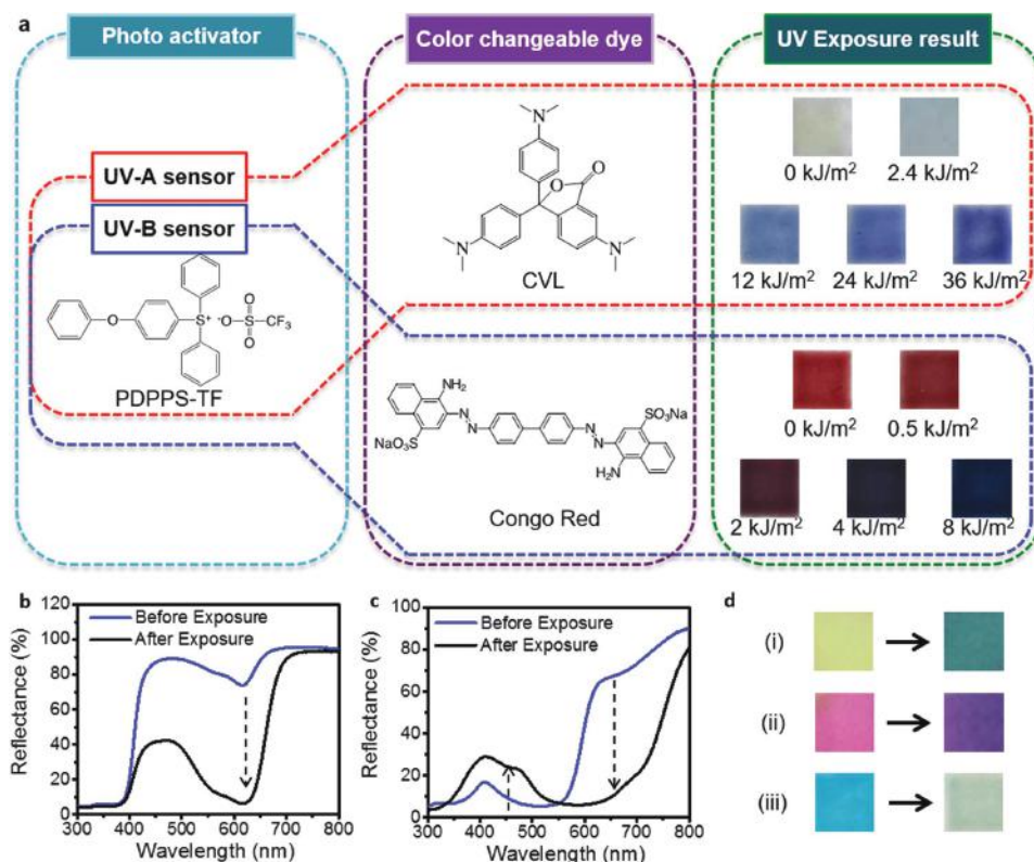
Figure 2. Chemistry and response of stretchable materials for colorimetric UV dosimetry. a) Chemical structure and the result of UV exposure. PPDPS-TF and CVL provide for sensing in the UV-A band. PPDPS-TF and Congo red provide for sensing in the UV-B band. b) UV-vis reflection spectra of PPDPS-TF and CVL mixed into a PDMS matrix, before and after exposure (thickness = 30 \mu\text{m} , exposure time = 10 min (by UV-A lamp, intensity = 22 \text{W m}^{-2} )). c) UV-vis reflection spectra of PPDPS-TF and Congo red mixed into a PDMS matrix before and after exposure (thickness = 30 \mu\text{m} , exposure time = 10 min (by UV-B lamp, intensity = 5 \text{W m}^{-2} )). d) Color diversity enabled by these chemistries. The left side is before exposure and the right side is after exposure. (i) Yellow to green transition associated with a material that consists of PPDPS-TF, CVL, and yellow pigment, with exposure condition identical to that in (b). (ii) Magenta to violet transition associated with a material that consists of PPDPS-TF and CVL and magenta pigment, with exposure condition identical to that in (b). (iii) Blue to colorless transition associated with a material that consists of Direct Blue 86 and Irgacure 2959, with exposure condition identical to that in (c).
