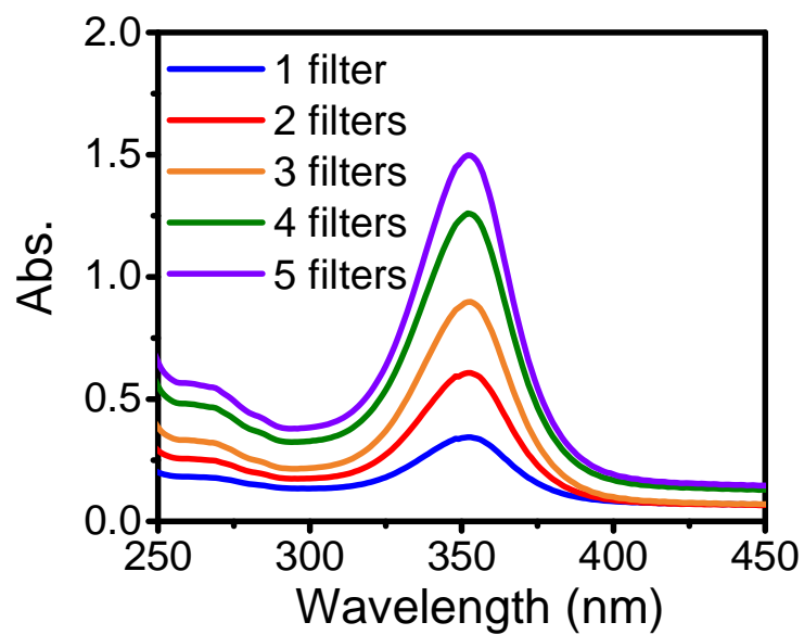
Figure S9 UV-vis absorption spectra of UV-A absorptive filters for experimental demonstrations of sensitivity control presented in Figure 3e.
