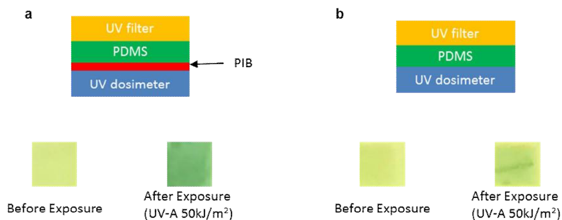
Figure S14 Schematic illustration and experimental results for the intermediate layer. a. Schematic illustration of the sample (top) and image before and after exposure (bottom) with or b. without the PIB intermediate layer.
