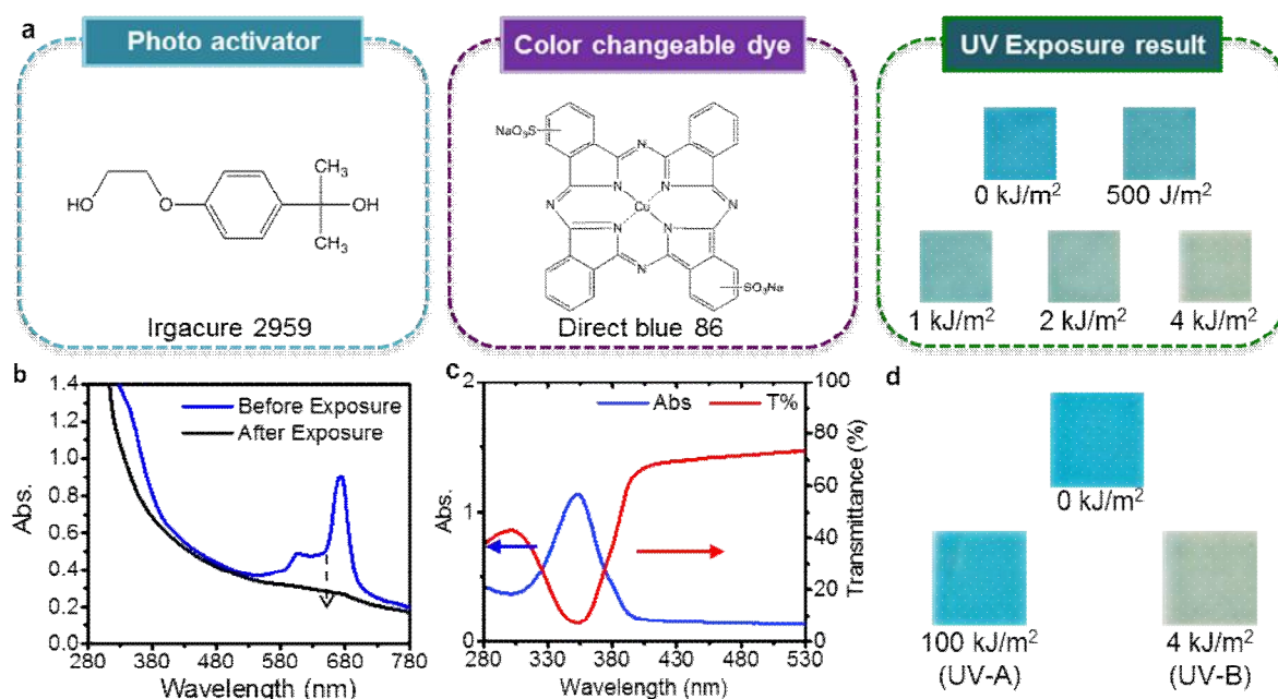
Figure S7. Chemistry and experimental results from UV colorimetric dosimetry materials. a. Chemical structure and colorimetric response of material formed with Irgacure 2959 and Direct blue 86. b. UV-vis absorption spectra of PDMS film mixed with Irgacure 2959 and Direct Blue 86 before and after exposure (Thickness = 30 \mu\text{m} ). c. UV spectra d. Color diversity of colorimetric material (i) colorless to red (made from PPDPS-TF, 6'-(Diethylamino)-1',2'-benzofluoran). (ii) yellow to green (made from PPDPS-TF, CVL, yellow pigment). (iii) magenta to violet (made from PPDPS-TF, CVL, Magenta pigment).
