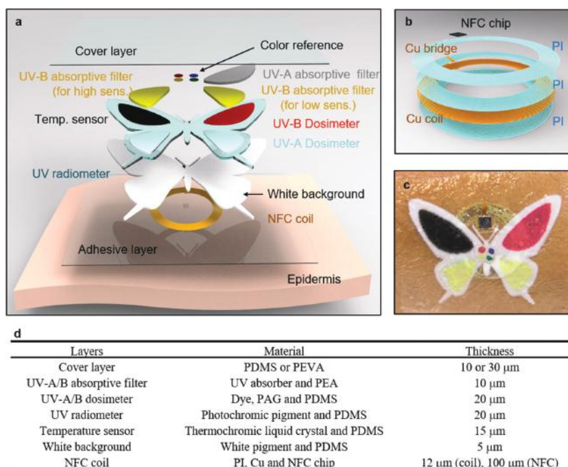
Figure 1. Schematic illustrations and digital image of a multimodal, colorimetric epidermal device with capabilities in UV and temperature sensing and in wireless operation via near field communication (NFC) electronics. a) Exploded-view schematic illustration of the various functional layers in a representative system. b) Schematic illustration of the NFC electronics, including an integrated temperature sensor. c) Image of a device on the skin. d) Table of materials and thicknesses for each layer in this system.
