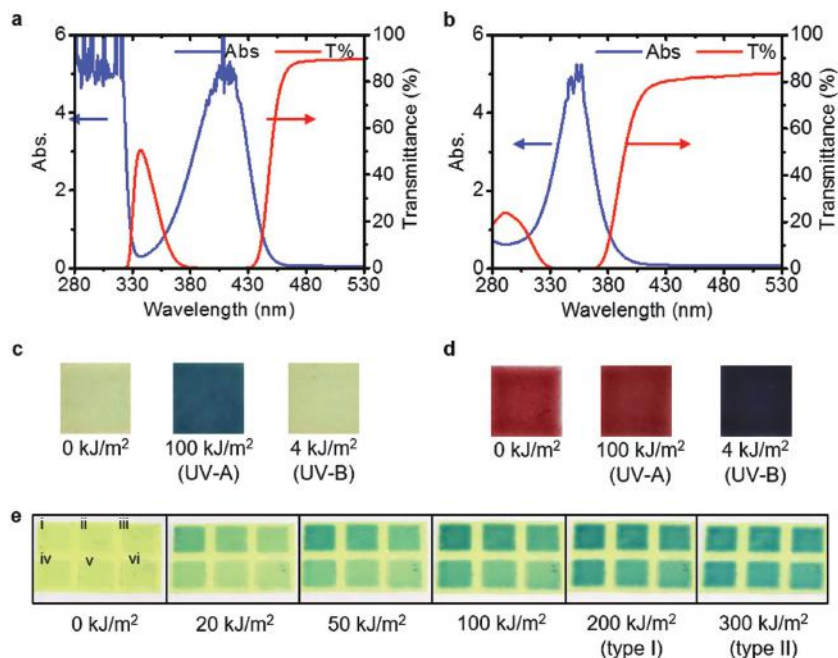
Figure 3. Experimental results for the behaviors of UV-A and UV-B stretchable colorimetric dosimeter materials and sensitivity control. UV-vis absorption spectra of a) UV-B and violet light absorptive filters and b) UV-A absorptive filter. Digital images of c) UV-A dosimeter and d) UV-B dosimeter before and after exposure using UV-A and UV-B lamps. e) 3 \times 2 array of UV-A dosimeter materials with or without a UV-A absorptive filter to control the sensitivity: (i) no filter, (ii)–(vi) 1–5 UV-A absorptive filters (Figure S9, Supporting Information).
