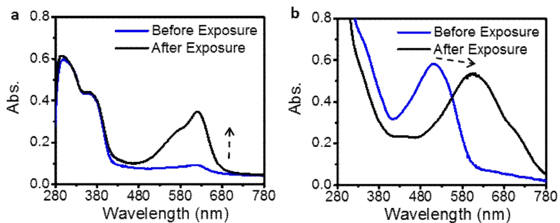
Figure s15 UV absorption spectra of UV colorimetric material
