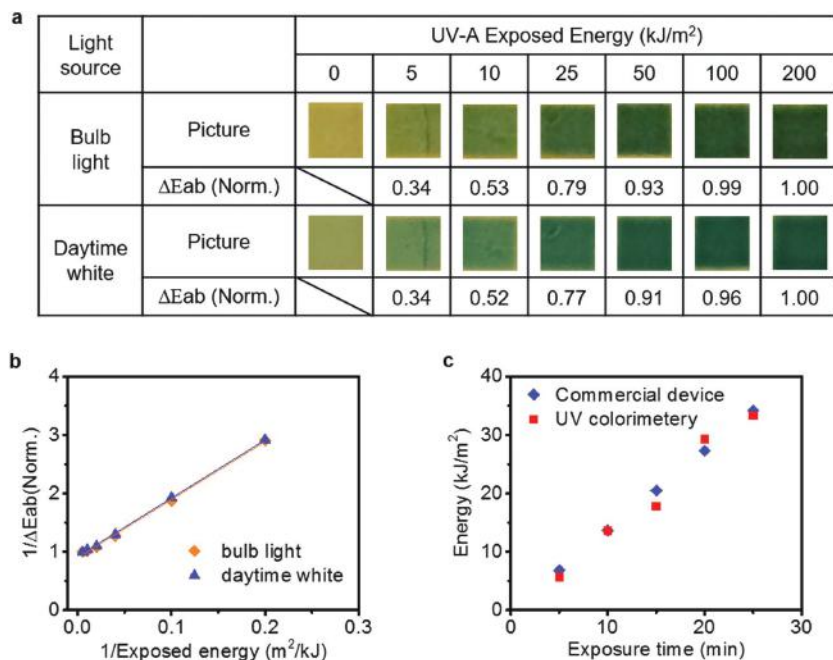
Figure 4. Methods for image analysis to determine the exposure dose from changes in color. a) Image and normalized value of \Delta Eab for the UV-A colorimetric dosimeter material after exposure with various energies ( \Delta Eab_x(\text{Norm.}) = \Delta Eab_x/\Delta Eab_{200} ). The images here were collected under incandescent light and daylight white fluorescent light. b) Plot of 1/x ( x = exposed energy) versus 1/\Delta Eab_x (Norm.). c) Results for UV measurement of sunlight in Urbana, IL, USA (at 2/27/2016 11:40–12:00 weather condition was sunny) using a commercial device and the UV colorimetric material. Calibration of the material was performed using a solar simulator (Newport).
