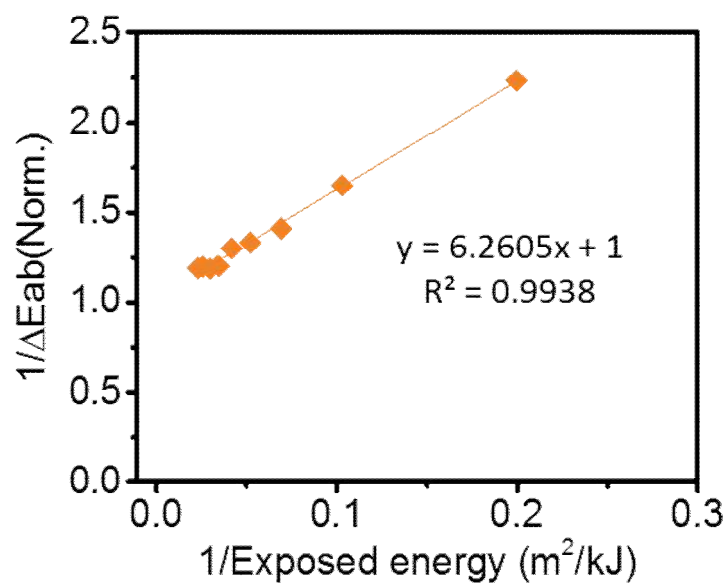
Figure S5 Calibration data. Plot of 1/\Delta E_{ab} vs 1/x ( x =exposed energy) for UV-A colorimetric dosimeter material under exposure using a solar simulator. The line defines the calibration.
