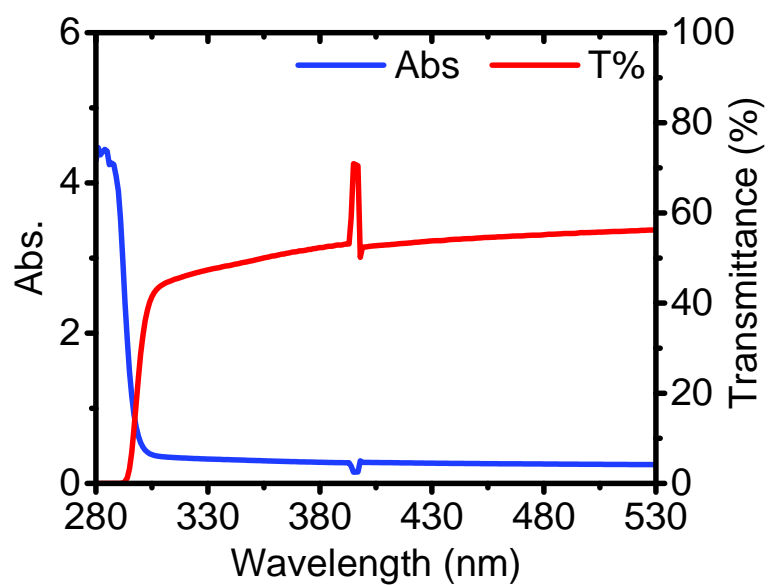
Figure S6 UV-vis absorption spectra of polyurethane (PU) film.
