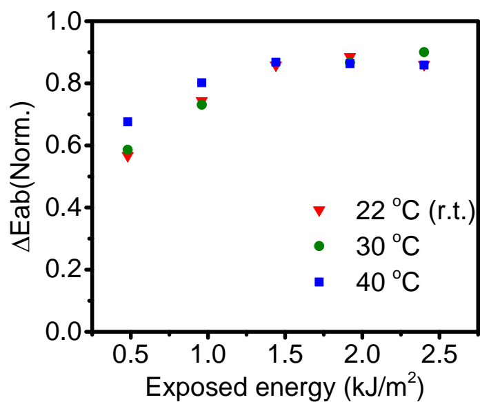
Figure S8. Temperature dependence of the response of UV colorimetry dosimetry material. Plot of exposed energy (=x) vs \Delta E_{ab} (Norm.) exposed with a solar simulator while on a hot plate at various temperatures (22 °C, 30 °C, 40 °C).
